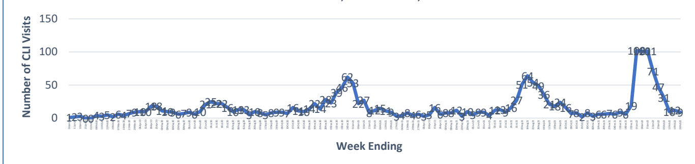
COVID-19-Like Illness (CLI) Visits Leake County, Mississippi Jan. 04, 2020 - Feb. 26, 2022
