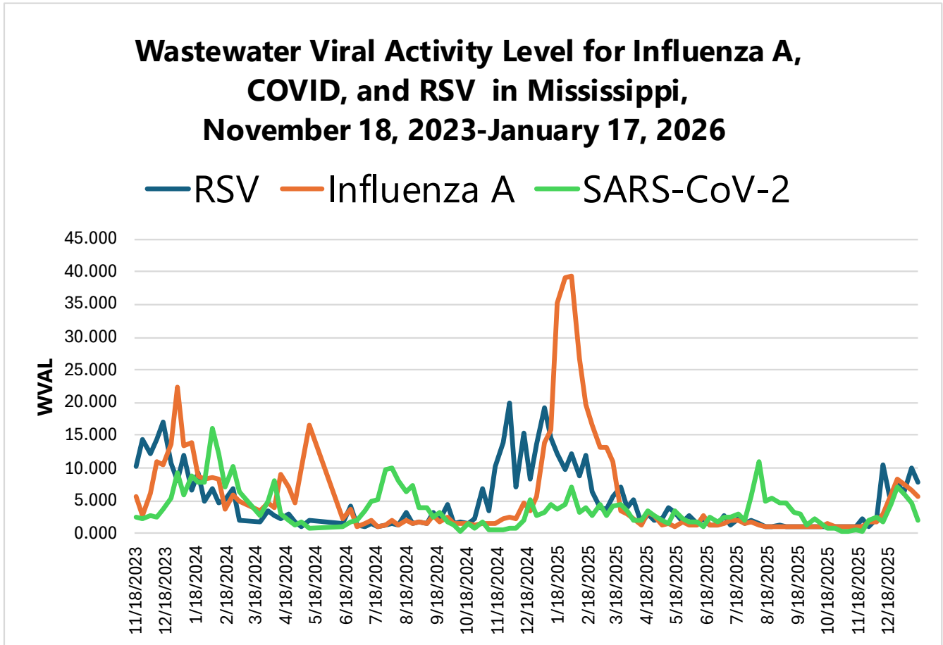
The Wastewater data shows a decrease in COVID RSV, and influenza A. | Figure 6
