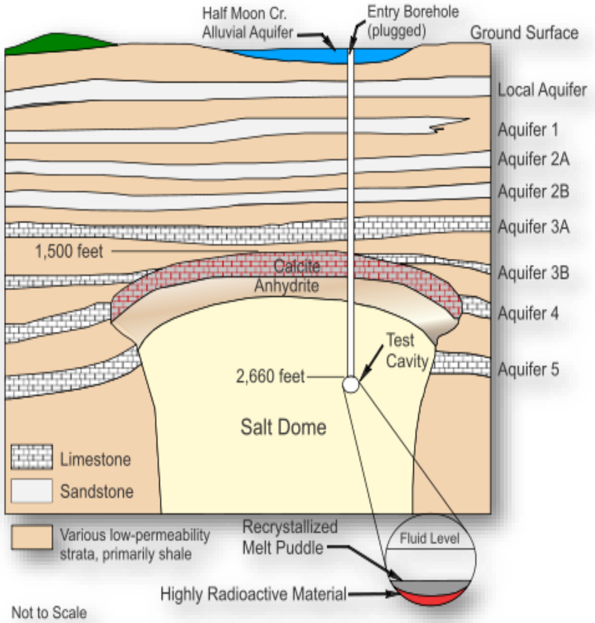
Figure 2, Test Cavity and Aquifers at the Salmon Test Site
